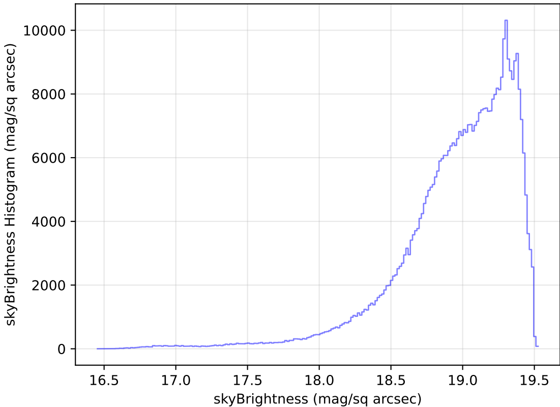
too_elab_r64_d2_gz_v3.4_10yrs All sky z band: skyBrightness Histogram
