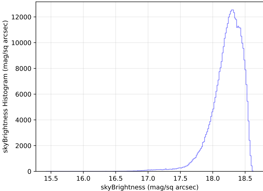
too_elab_r64_d2_gz_v3.4_10yrs All sky y band: skyBrightness Histogram
