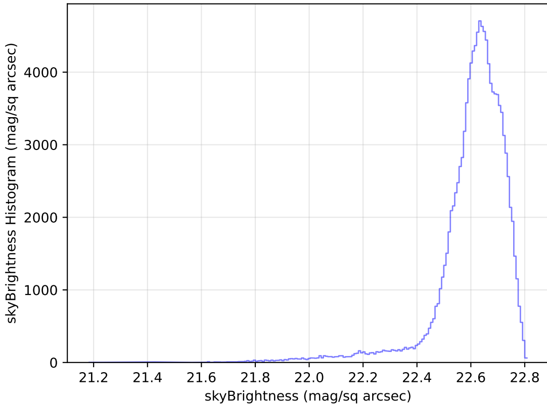
too_elab_r64_d2_gz_v3.4_10yrs All sky u band: skyBrightness Histogram
