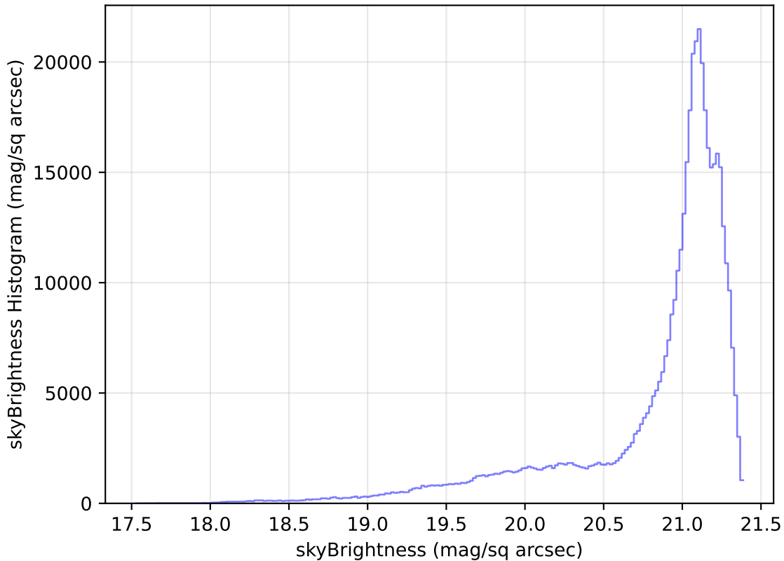
too_elab_r64_d2_gz_v3.4_10yrs All sky r band: skyBrightness Histogram
