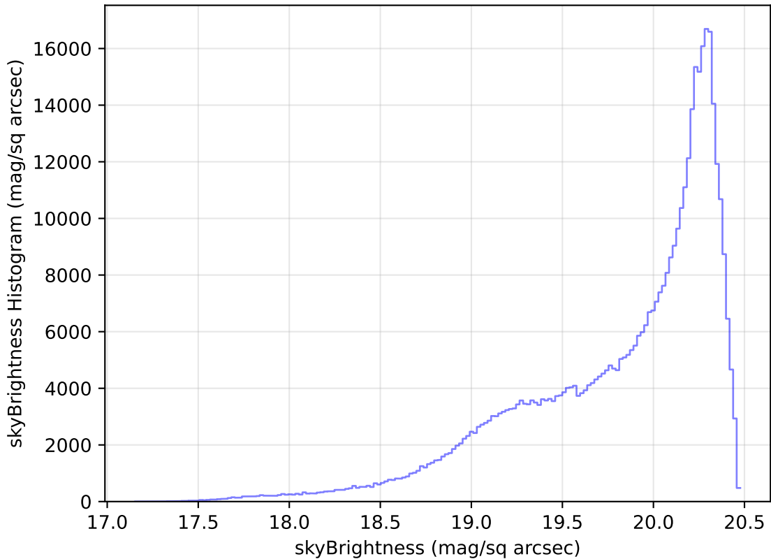
too_elab_r64_d2_gz_v3.4_10yrs All sky i band: skyBrightness Histogram
