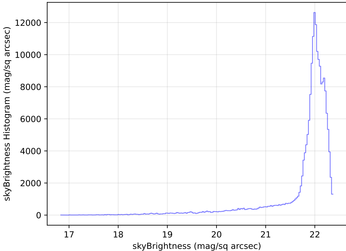
too_elab_r64_d2_gz_v3.4_10yrs All sky g band: skyBrightness Histogram
