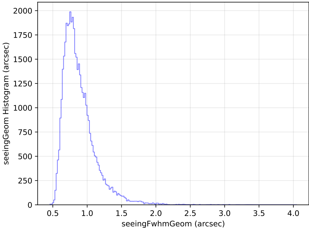
too_elab_r64_d2_gz_v3.4_10yrs Yr 1 z band: seeingGeom Histogram
