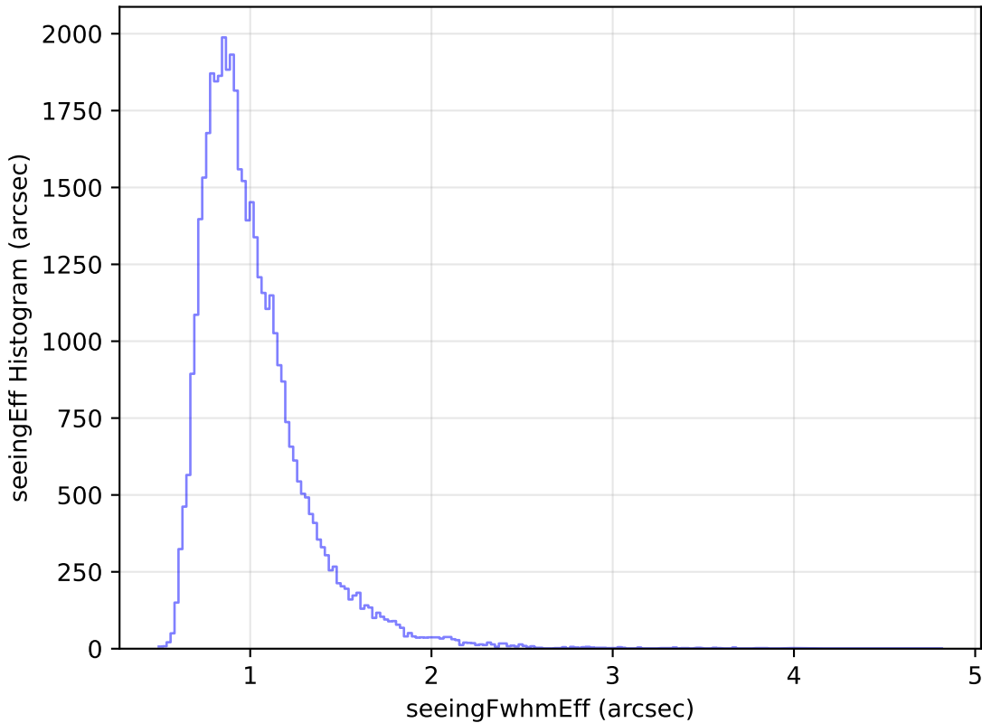
too_elab_r64_d2_gz_v3.4_10yrs Yr 1 z band: seeingEff Histogram
