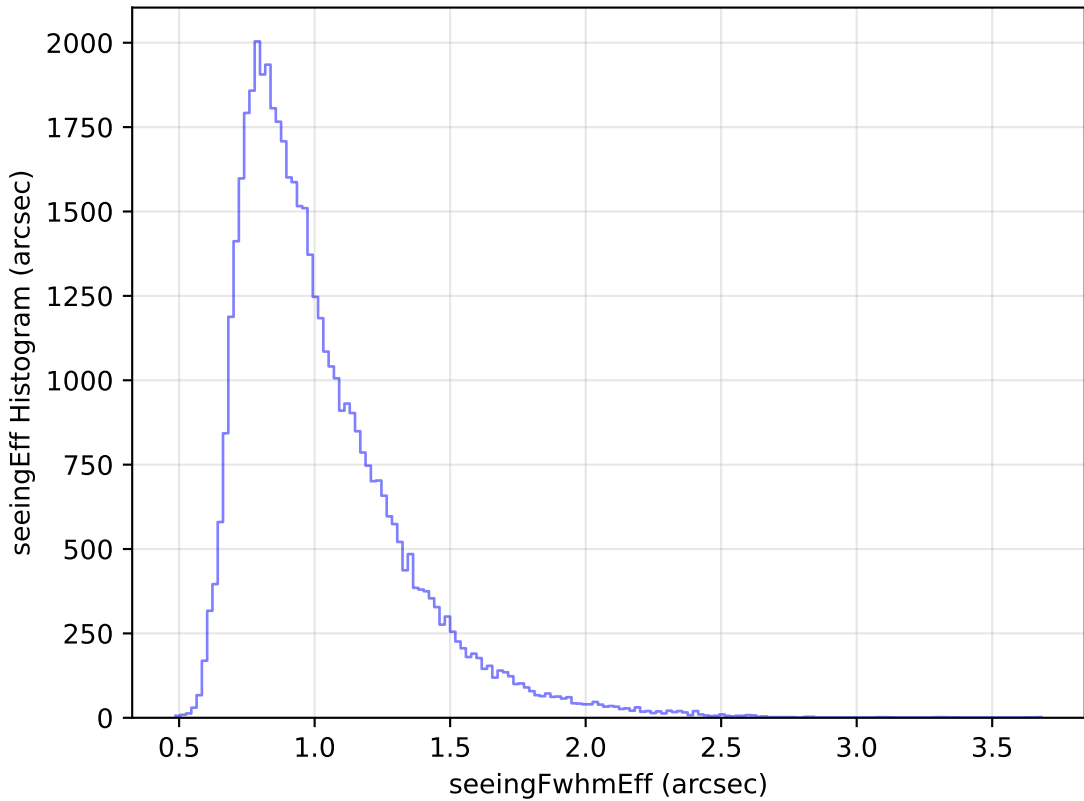
too_elab_r64_d2_gz_v3.4_10yrs Yr 1 r band: seeingEff Histogram
