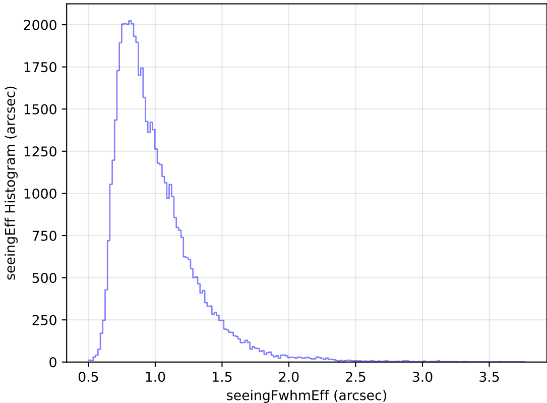
too_elab_r64_d2_gz_v3.4_10yrs Yr 1 i band: seeingEff Histogram
