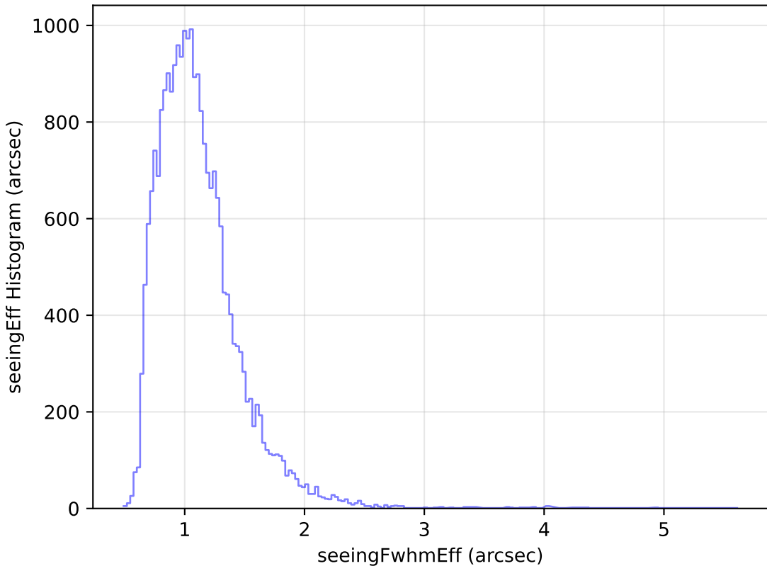
too_elab_r64_d2_gz_v3.4_10yrs Yr 1 g band: seeingEff Histogram
