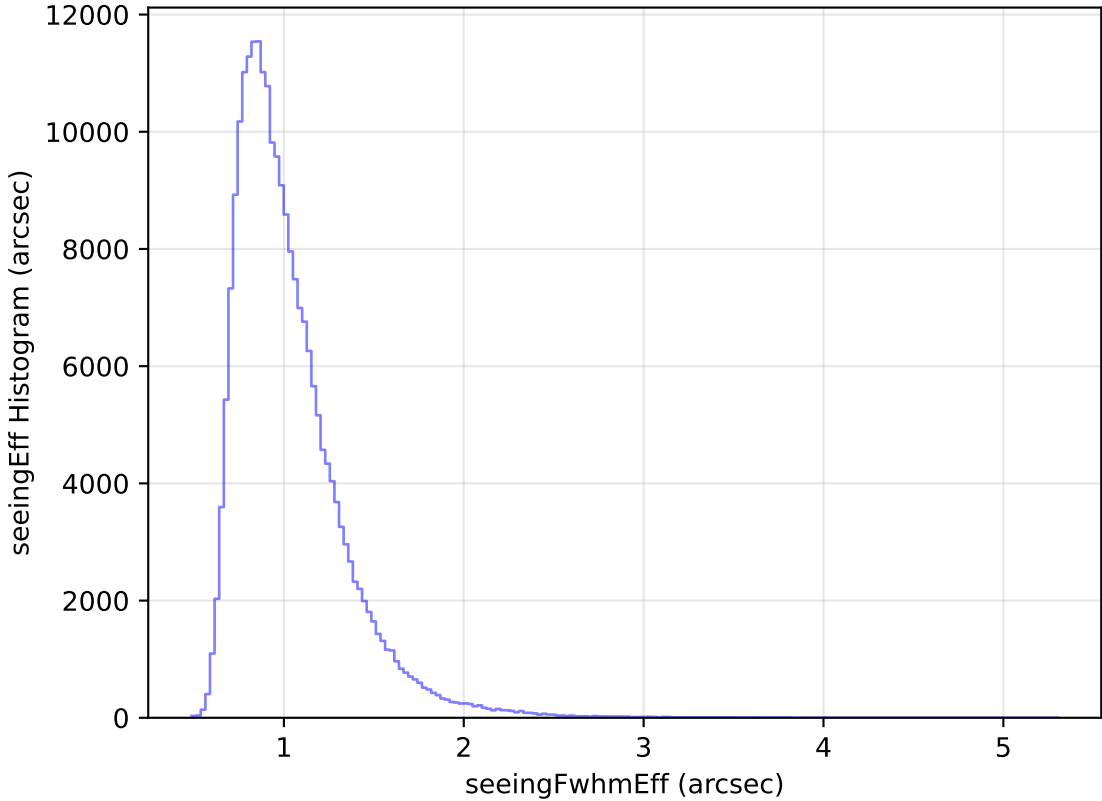
too_elab_r64_d2_gz_v3.4_10yrs Yr 1 all bands: seeingEff Histogram
