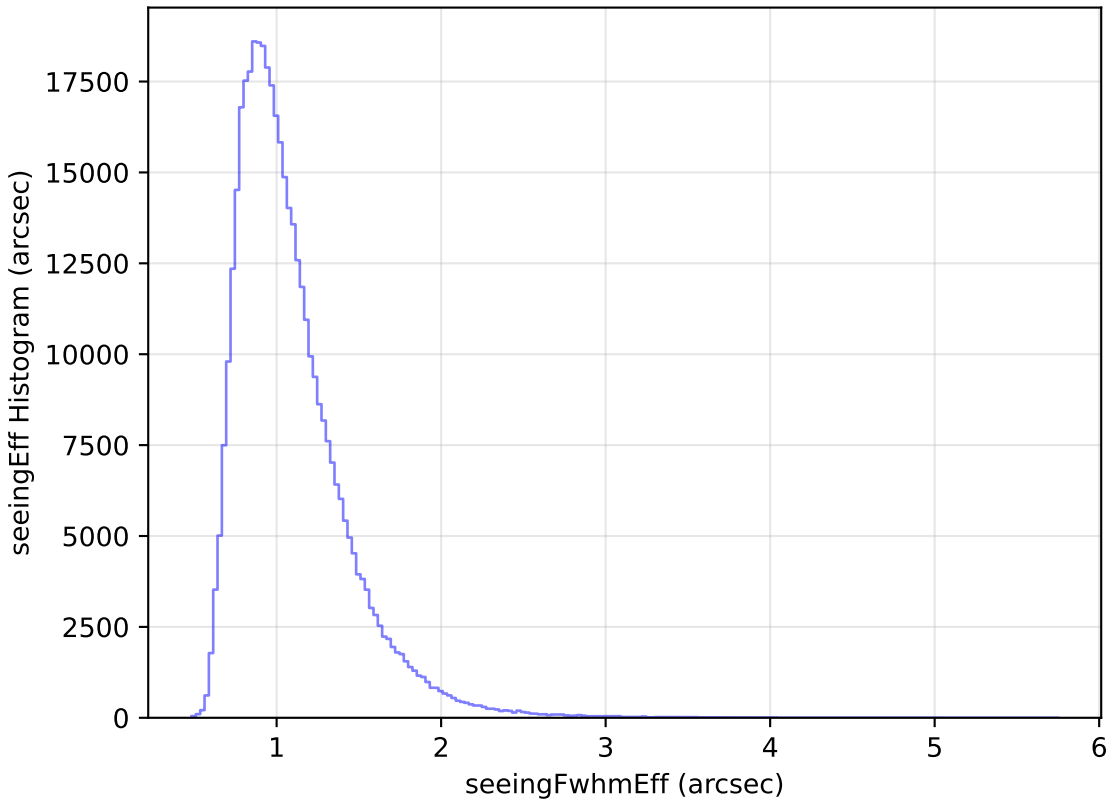
too_elab_r64_d2_gz_v3.4_10yrs WFD z band: seeingEff Histogram
