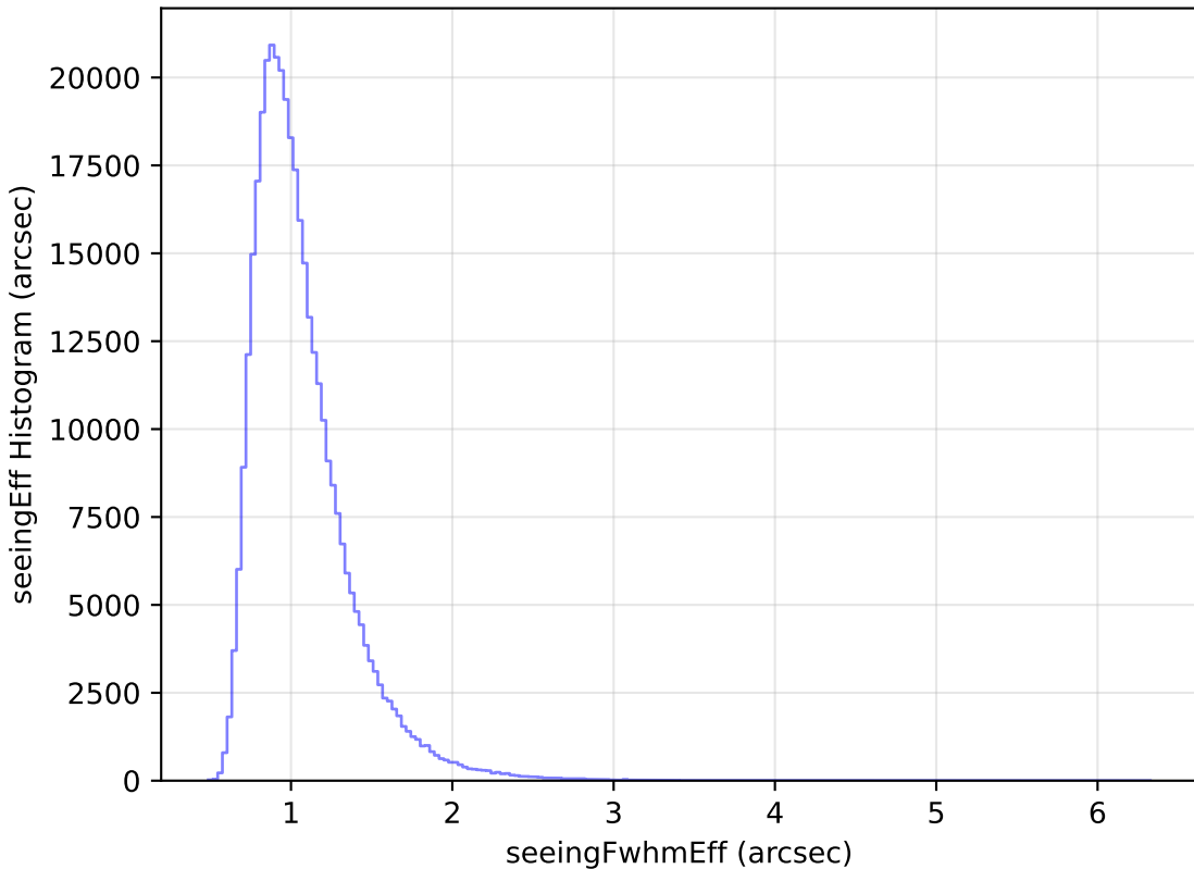
too_elab_r64_d2_gz_v3.4_10yrs WFD y band: seeingEff Histogram
