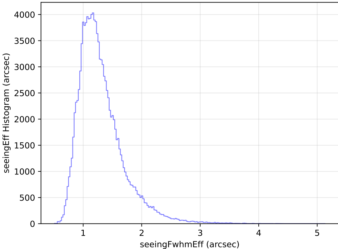
too_elab_r64_d2_gz_v3.4_10yrs WFD u band: seeingEff Histogram
