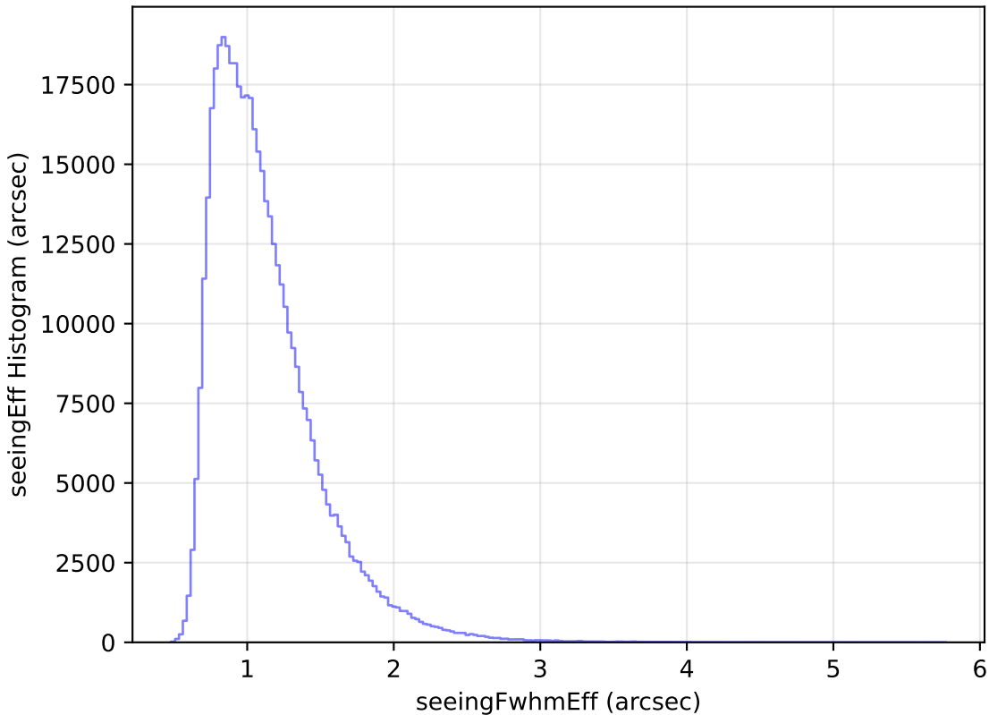
too_elab_r64_d2_gz_v3.4_10yrs WFD r band: seeingEff Histogram
