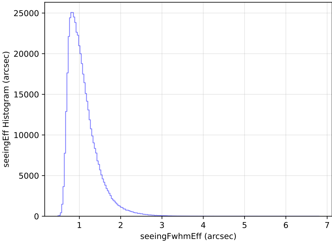
too_elab_r64_d2_gz_v3.4_10yrs WFD i band: seeingEff Histogram
