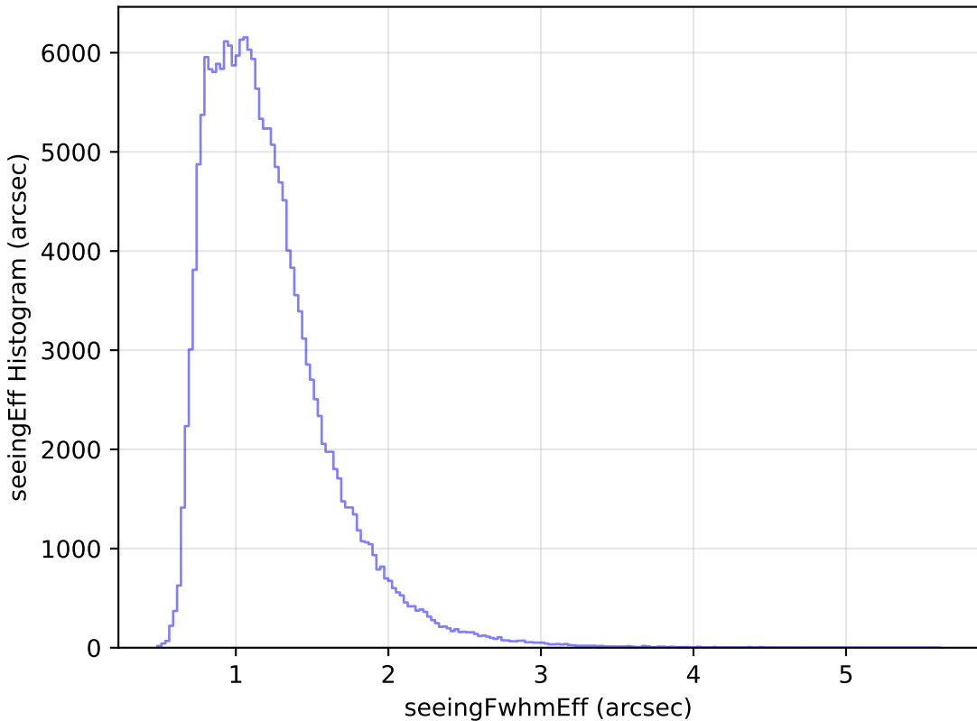
too_elab_r64_d2_gz_v3.4_10yrs WFD g band: seeingEff Histogram
