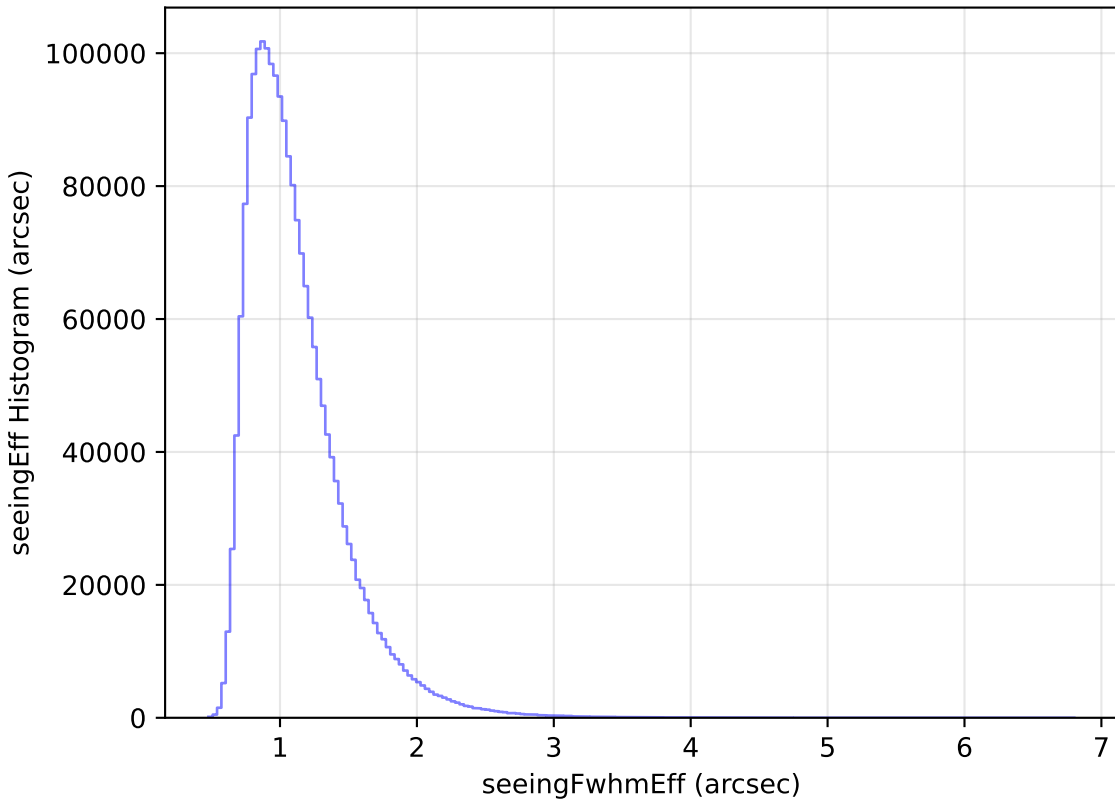
too_elab_r64_d2_gz_v3.4_10yrs WFD all bands: seeingEff Histogram
