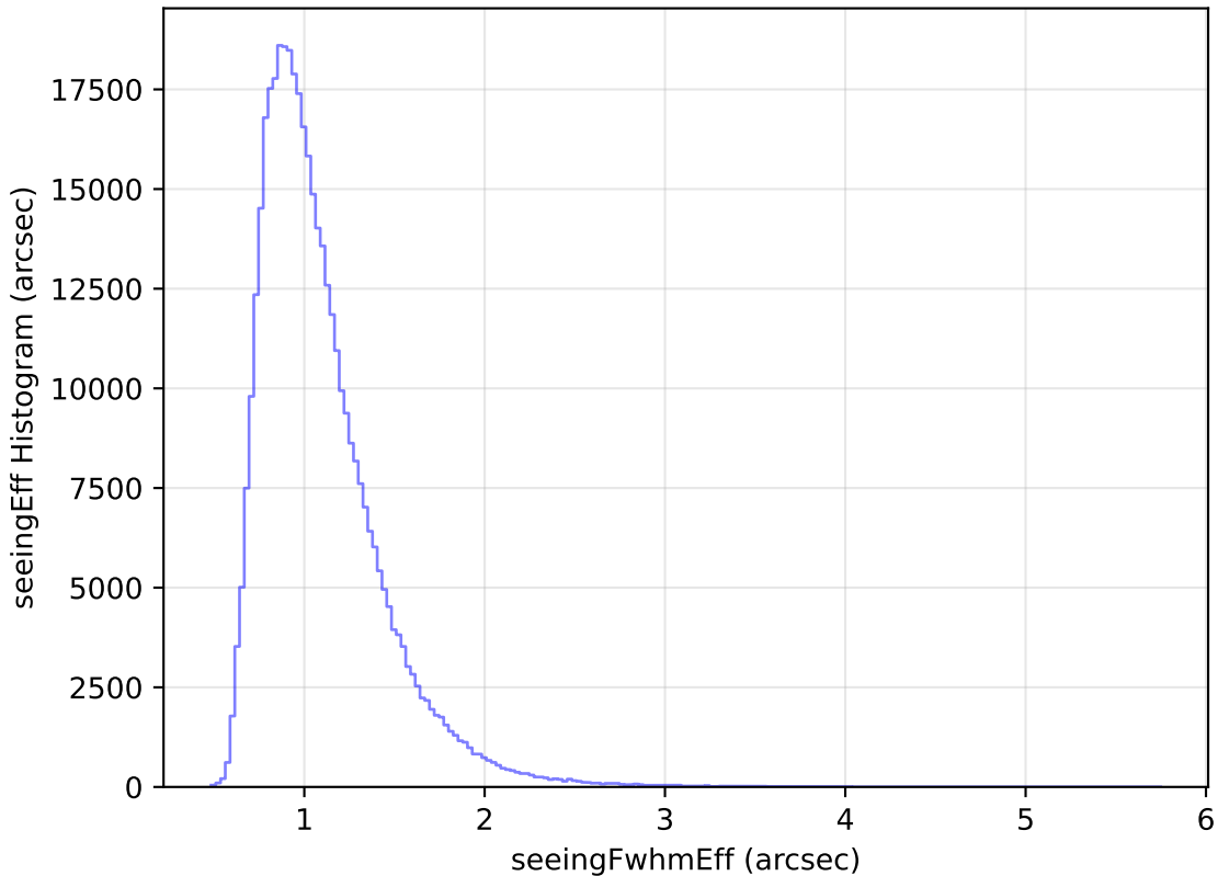
too_elab_r64_d2_gz_v3.4_10yrs All sky z band: seeingEff Histogram
