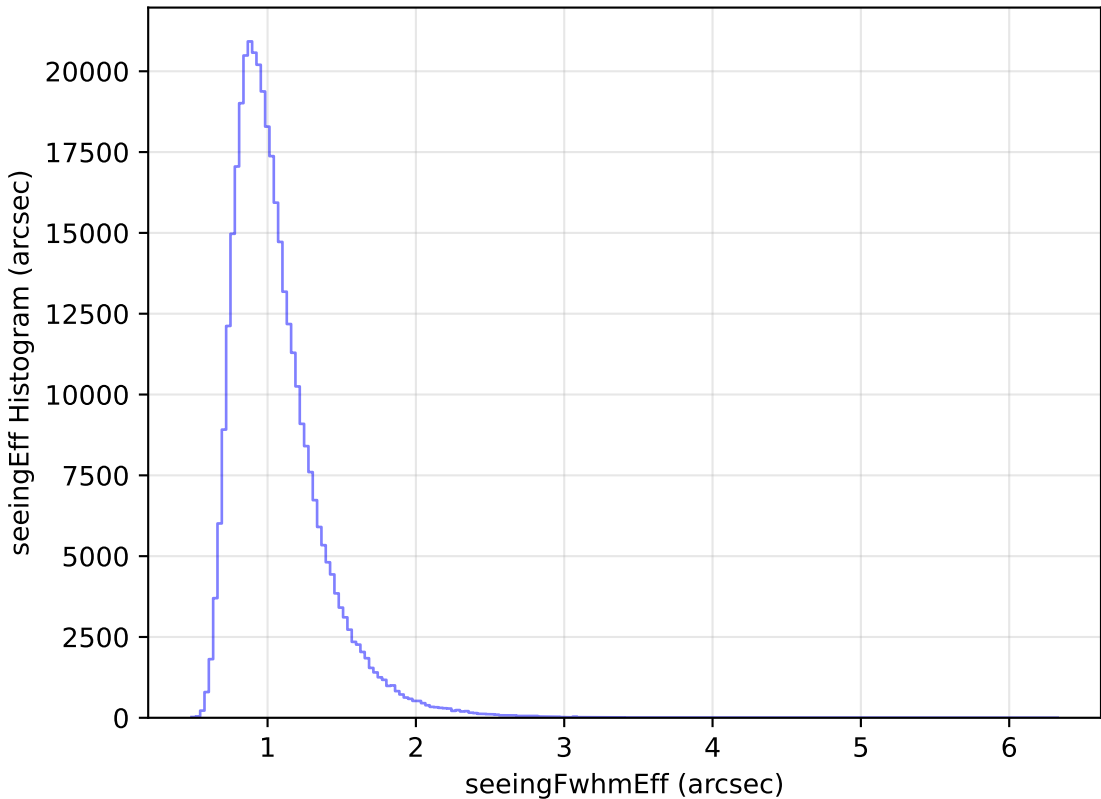
too_elab_r64_d2_gz_v3.4_10yrs All sky y band: seeingEff Histogram
