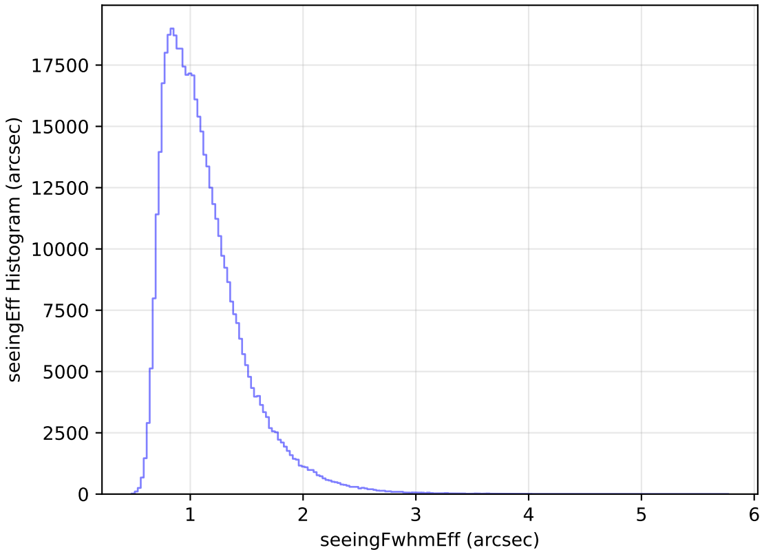
too_elab_r64_d2_gz_v3.4_10yrs All sky r band: seeingEff Histogram
