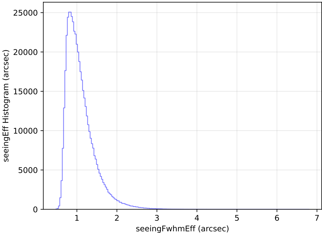
too_elab_r64_d2_gz_v3.4_10yrs All sky i band: seeingEff Histogram
