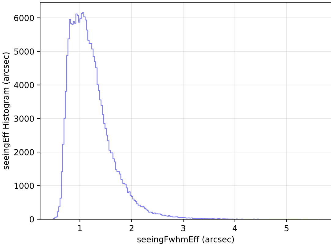
too_elab_r64_d2_gz_v3.4_10yrs All sky g band: seeingEff Histogram
