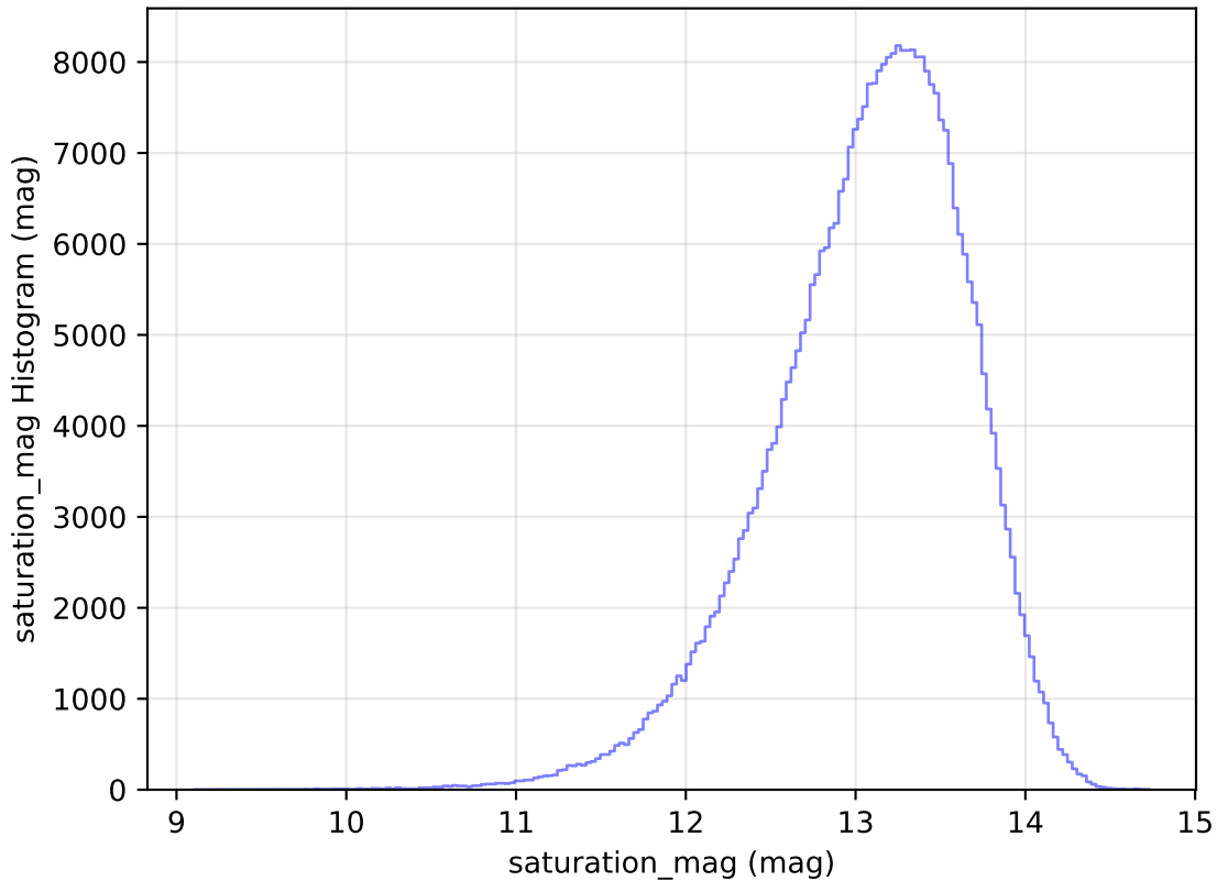
too_elab_r64_d2_gz_v3.4_10yrs WFD y band: saturation_mag Histogram
