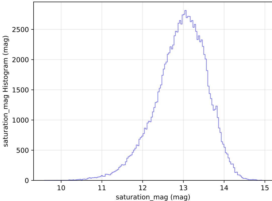
too_elab_r64_d2_gz_v3.4_10yrs WFD u band: saturation_mag Histogram
