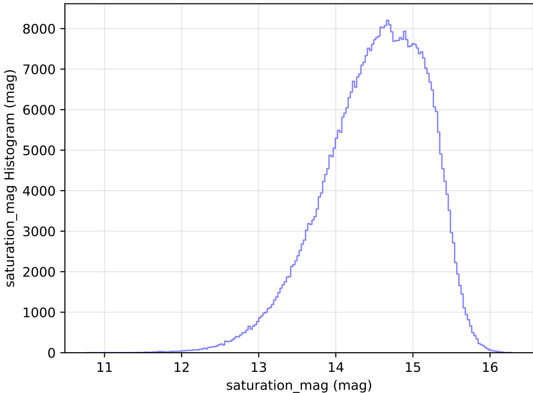
too_elab_r64_d2_gz_v3.4_10yrs WFD r band: saturation_mag Histogram
