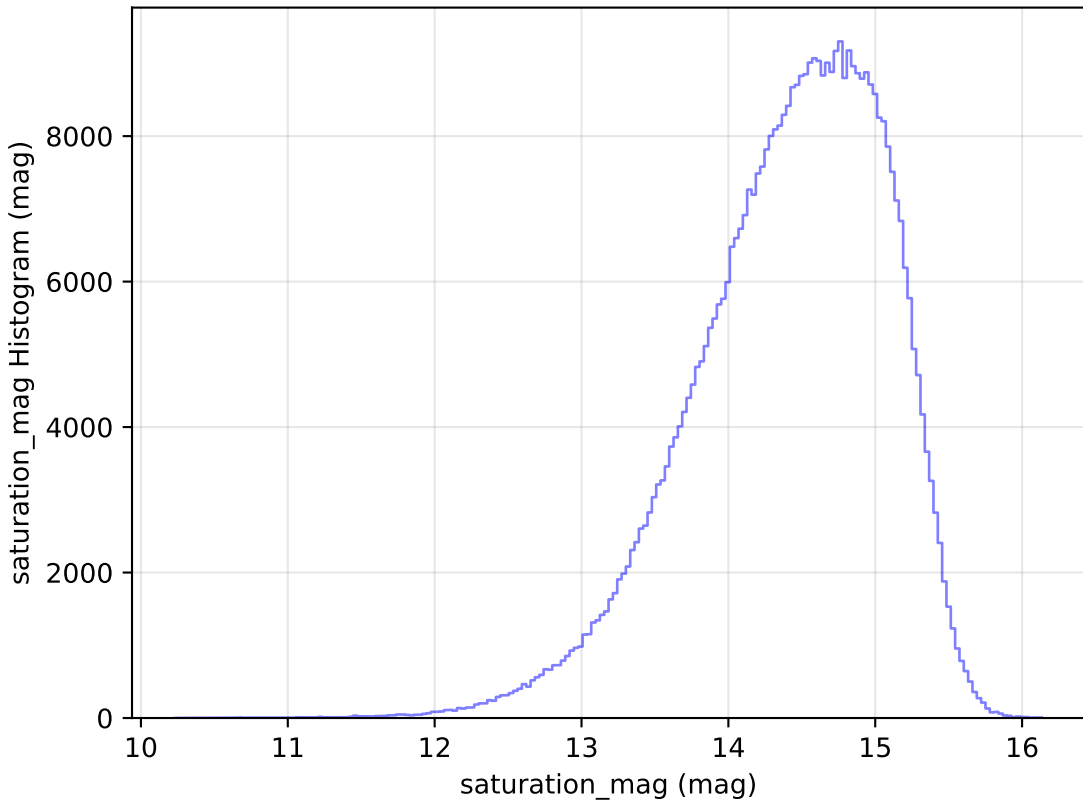
too_elab_r64_d2_gz_v3.4_10yrs WFD i band: saturation_mag Histogram
