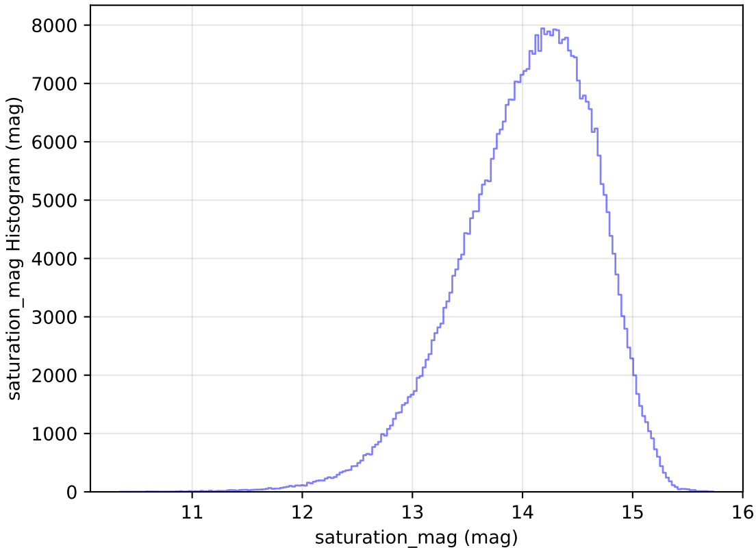
too_elab_r64_d2_gz_v3.4_10yrs All sky z band: saturation_mag Histogram
