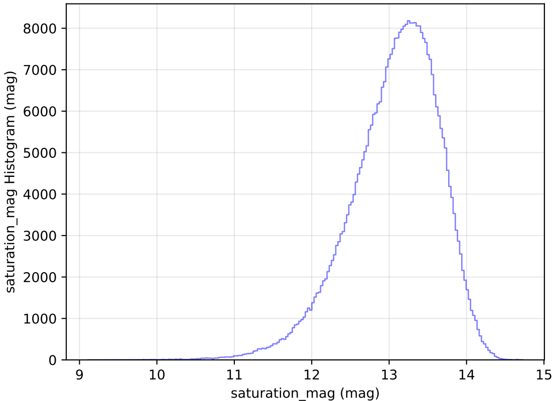
too_elab_r64_d2_gz_v3.4_10yrs All sky y band: saturation_mag Histogram
