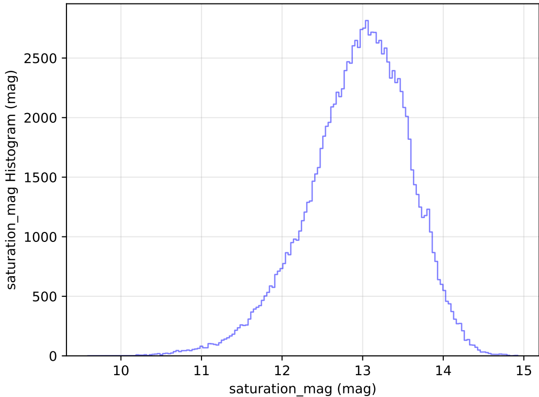
too_elab_r64_d2_gz_v3.4_10yrs All sky u band: saturation_mag Histogram
