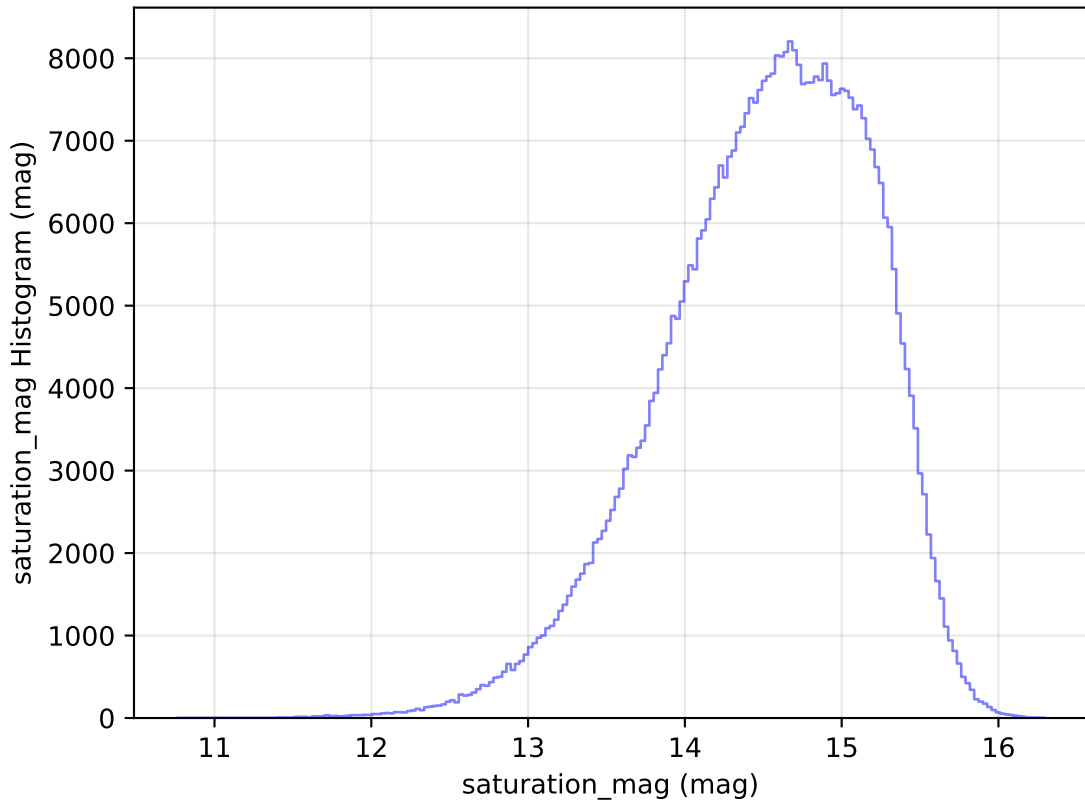
too_elab_r64_d2_gz_v3.4_10yrs All sky r band: saturation_mag Histogram
