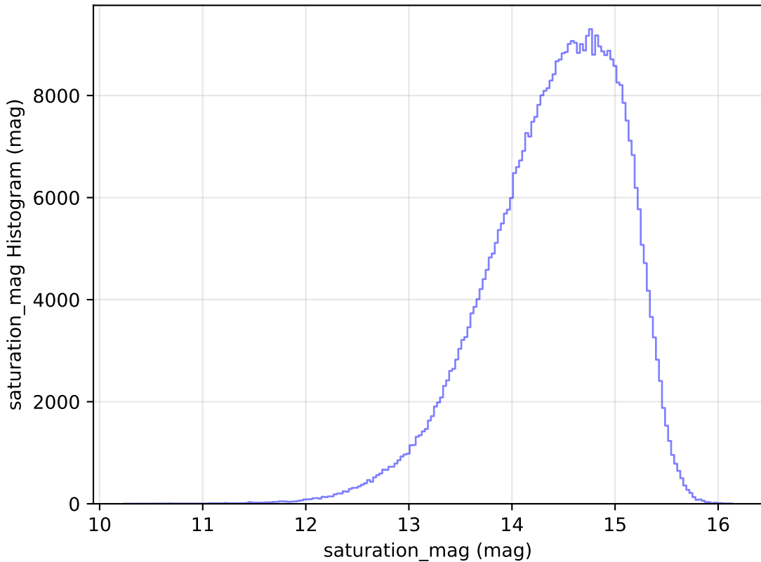
too_elab_r64_d2_gz_v3.4_10yrs All sky i band: saturation_mag Histogram
