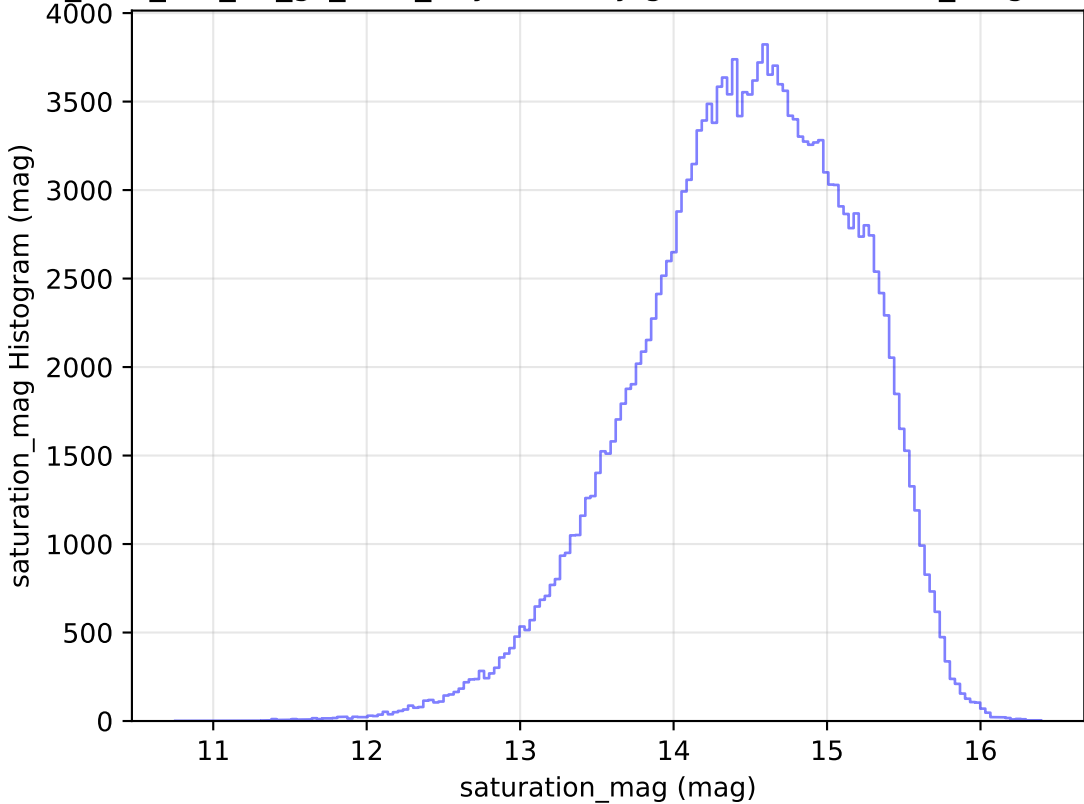
too_elab_r64_d2_gz_v3.4_10yrs All sky g band: saturation_mag Histogram
