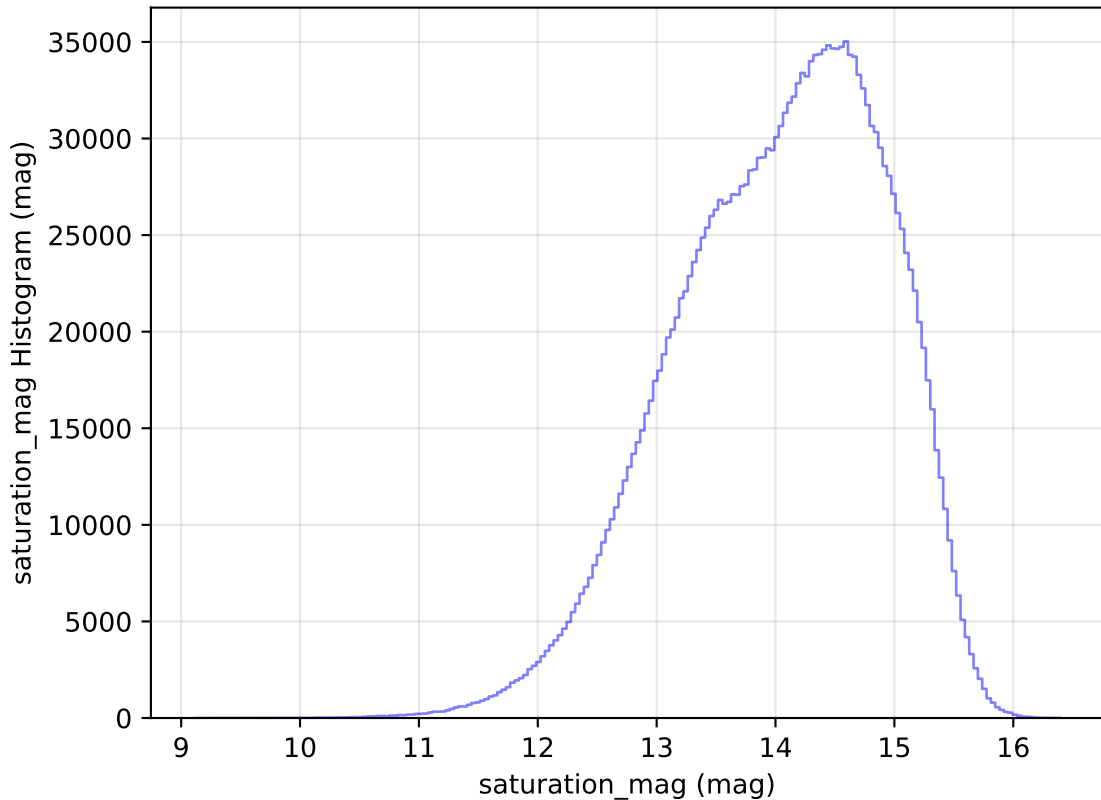
too_elab_r64_d2_gz_v3.4_10yrs All sky all bands: saturation_mag Histogram
