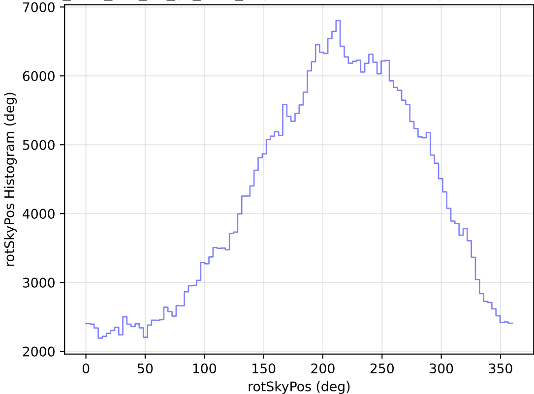
too_elab_r64_d2_gz_v3.4_10yrs WFD z band: rotSkyPos Histogram
