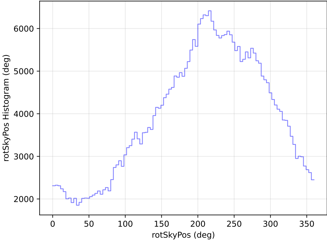
too_elab_r64_d2_gz_v3.4_10yrs WFD y band: rotSkyPos Histogram
