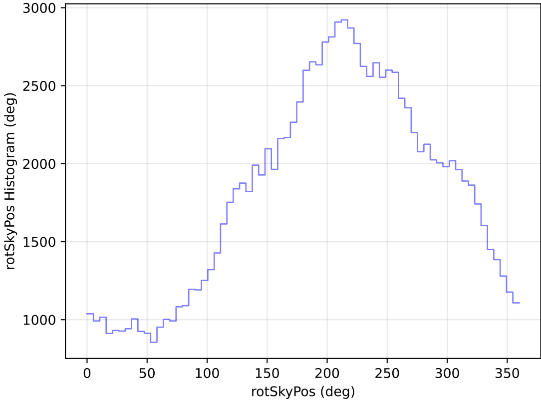
too_elab_r64_d2_gz_v3.4_10yrs WFD u band: rotSkyPos Histogram
