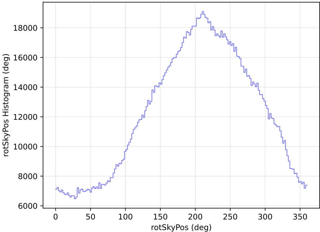
too_elab_r64_d2_gz_v3.4_10yrs WFD all bands: rotSkyPos Histogram
