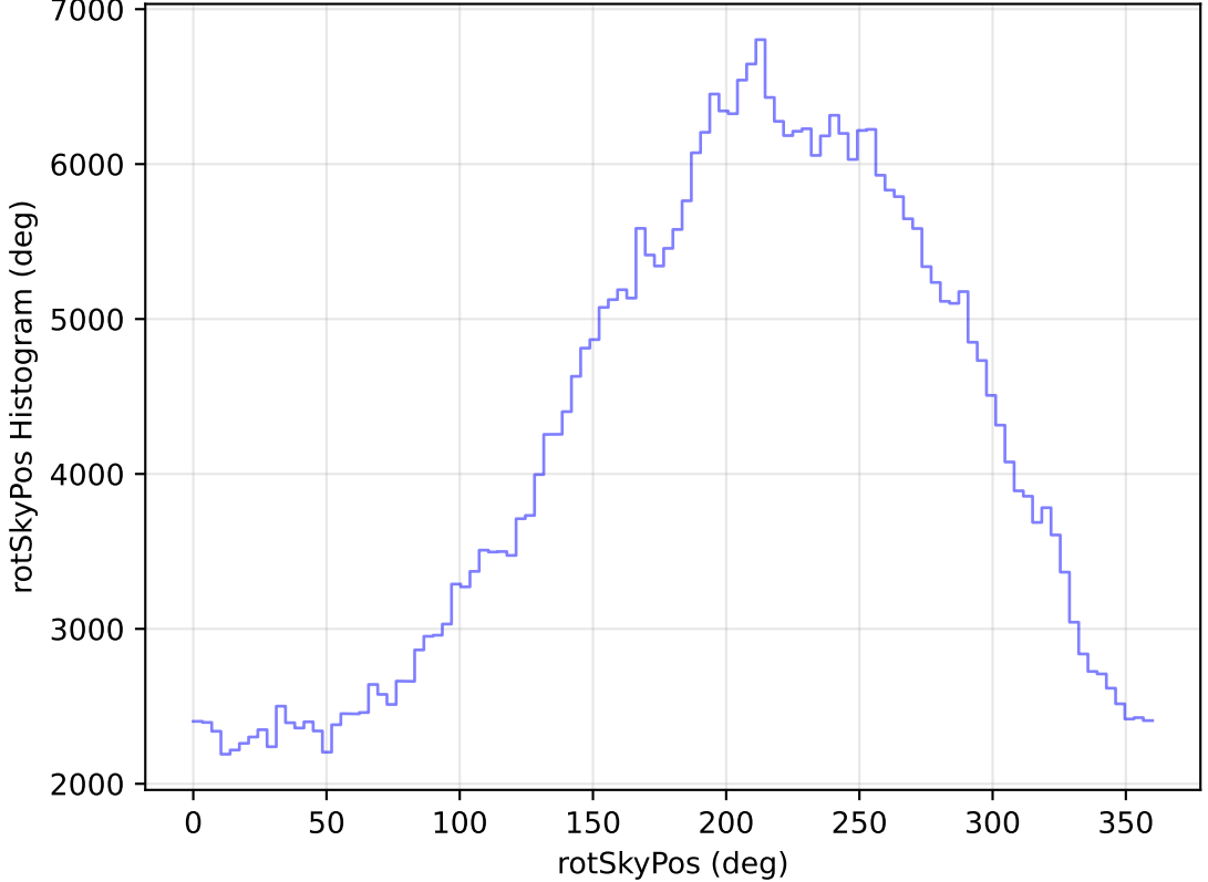
too_elab_r64_d2_gz_v3.4_10yrs All sky z band: rotSkyPos Histogram
