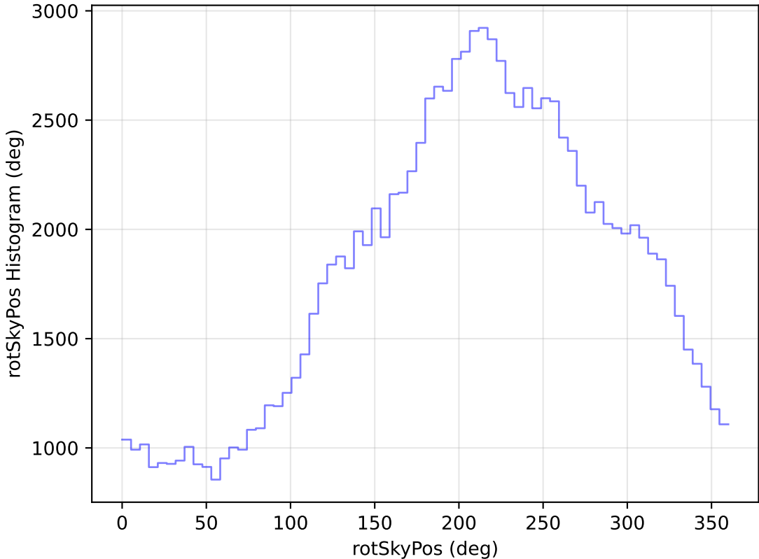
too_elab_r64_d2_gz_v3.4_10yrs All sky u band: rotSkyPos Histogram
