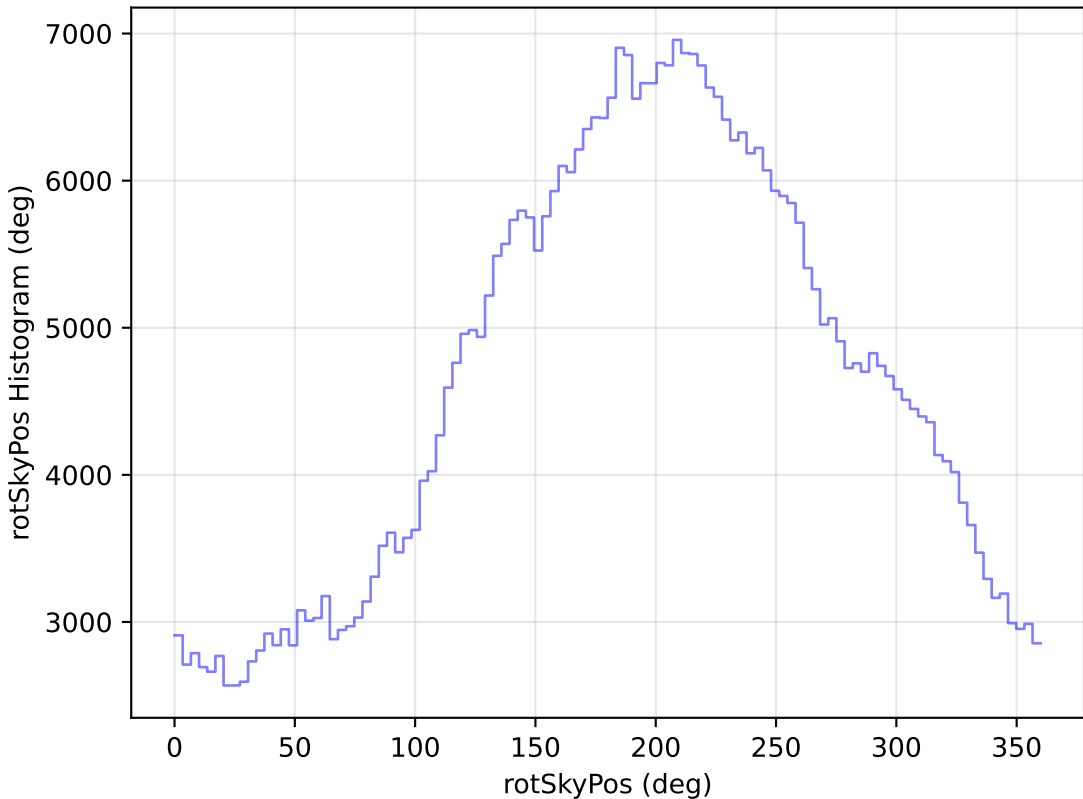
too_elab_r64_d2_gz_v3.4_10yrs All sky r band: rotSkyPos Histogram
