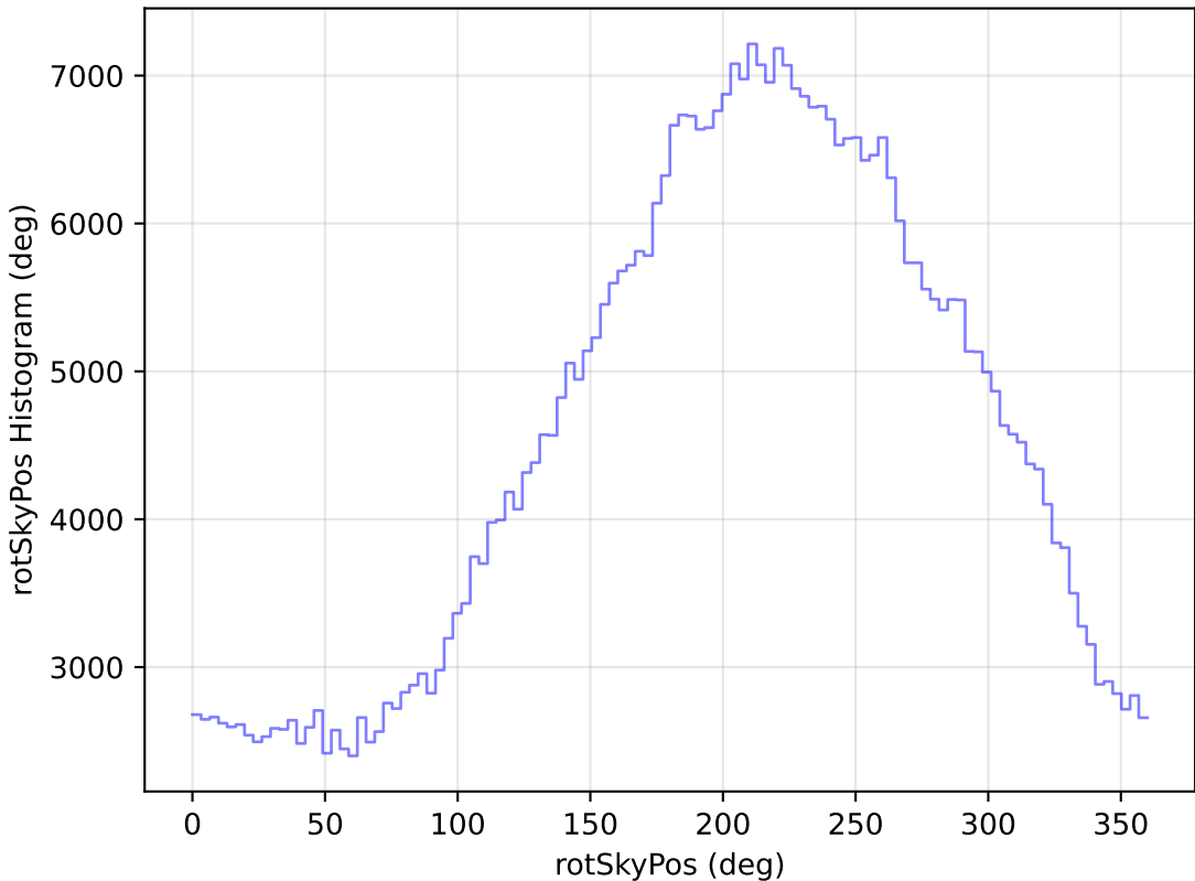
too_elab_r64_d2_gz_v3.4_10yrs All sky i band: rotSkyPos Histogram
