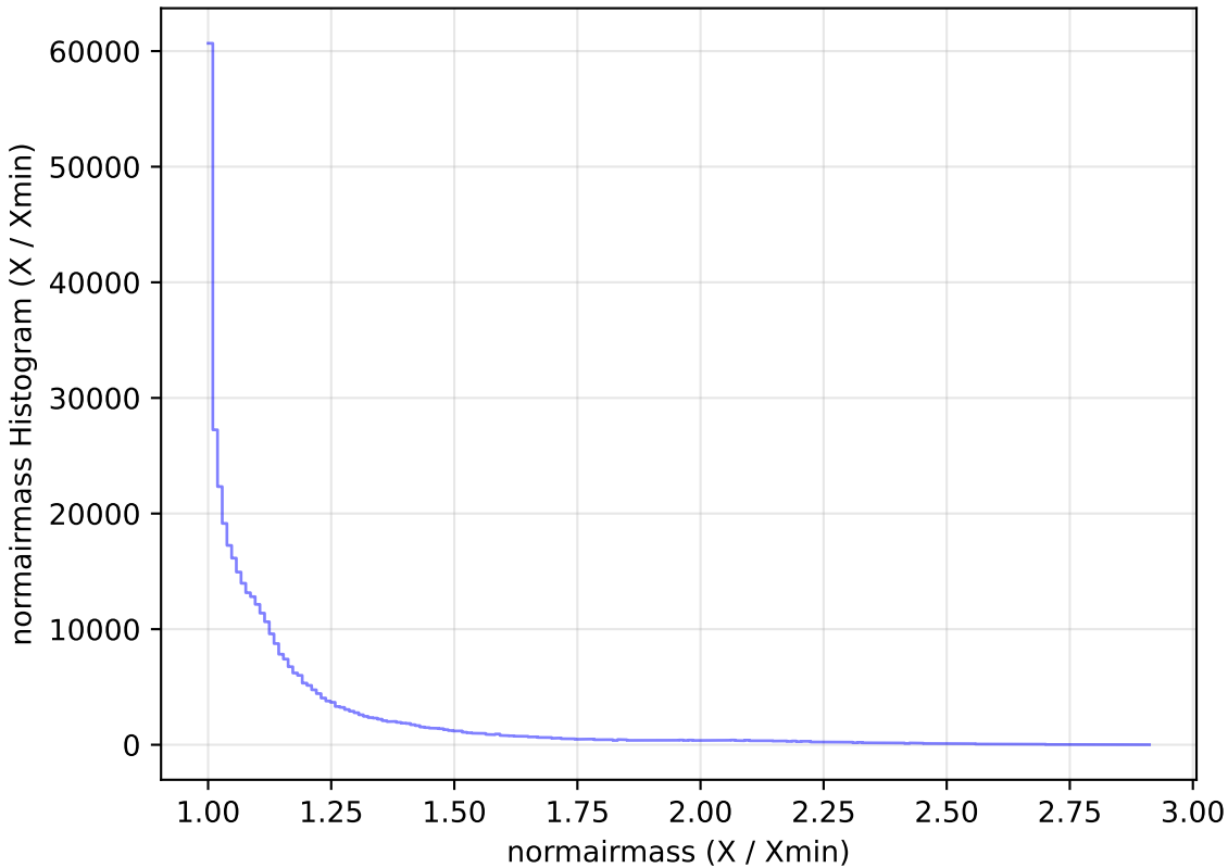
too_elab_r64_d2_gz_v3.4_10yrs WFD z band: normairmass Histogram
