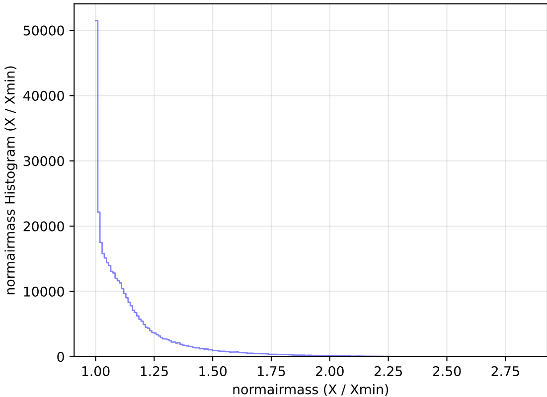
too_elab_r64_d2_gz_v3.4_10yrs WFD y band: normairmass Histogram
