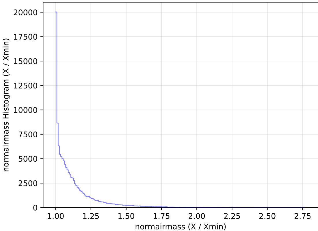
too_elab_r64_d2_gz_v3.4_10yrs WFD u band: normairmass Histogram
