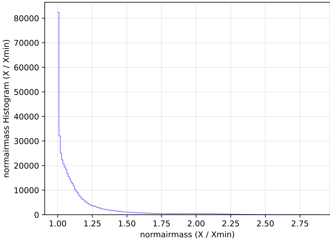
too_elab_r64_d2_gz_v3.4_10yrs WFD r band: normairmass Histogram
