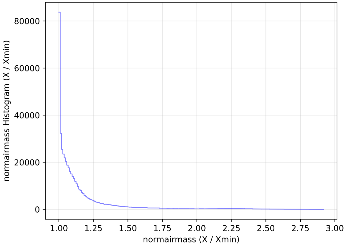
too_elab_r64_d2_gz_v3.4_10yrs WFD i band: normairmass Histogram
