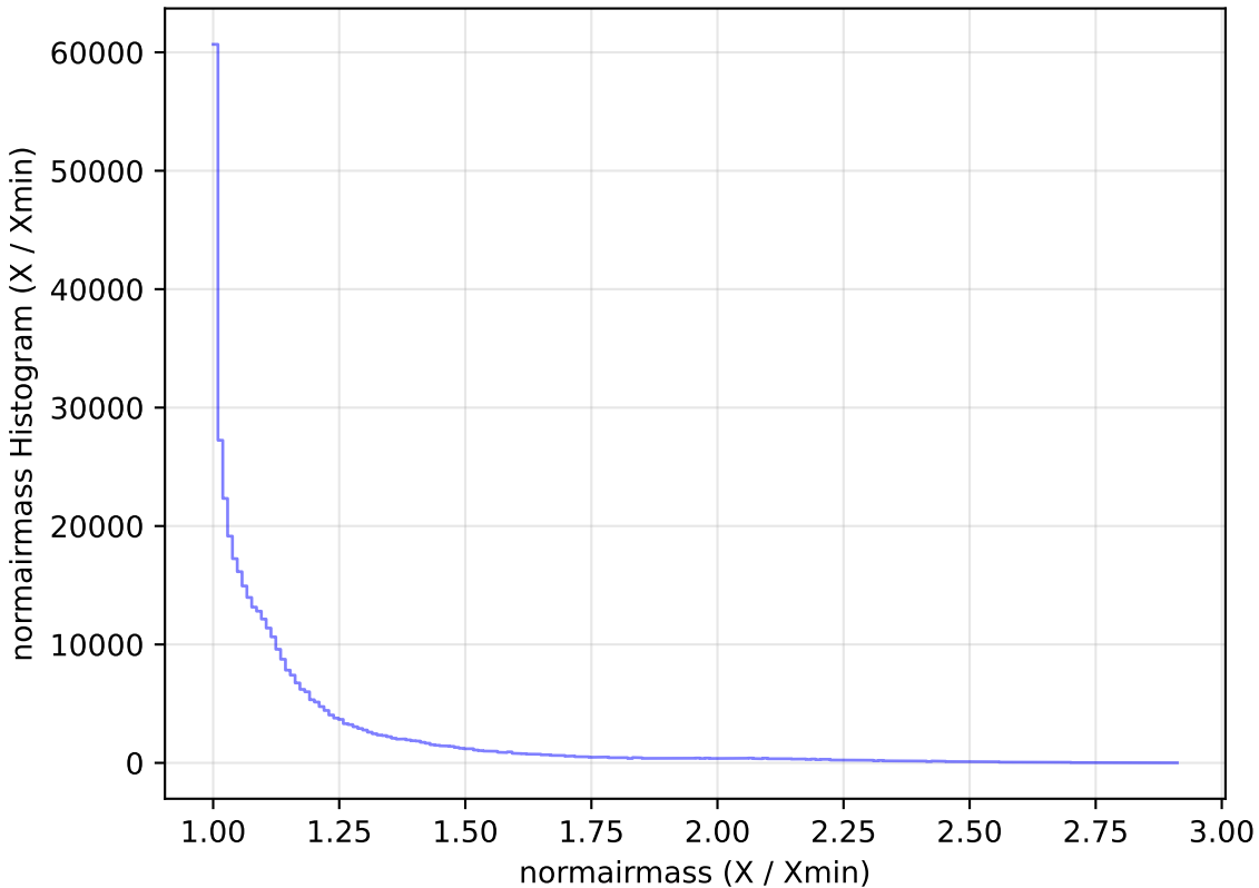
too_elab_r64_d2_gz_v3.4_10yrs All sky z band: normairmass Histogram
