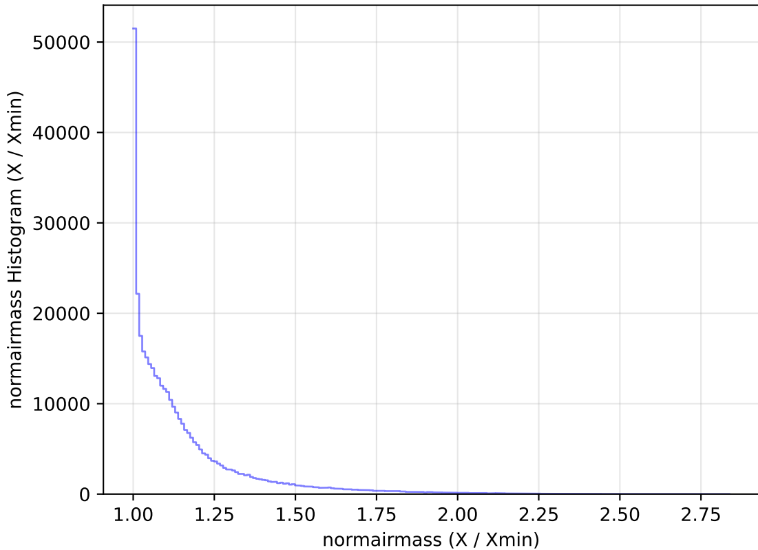
too_elab_r64_d2_gz_v3.4_10yrs All sky y band: normairmass Histogram
